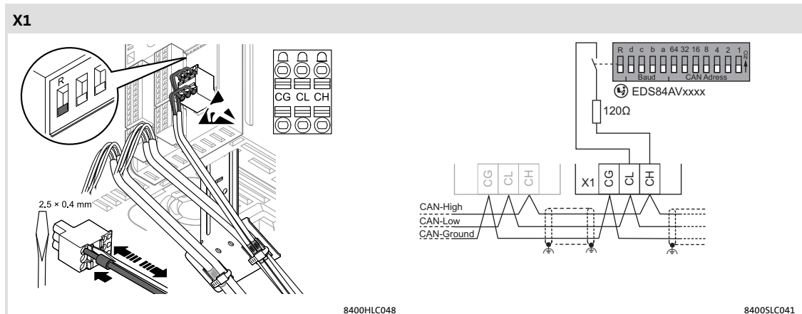
Fig. 6-29 CANopen connection
