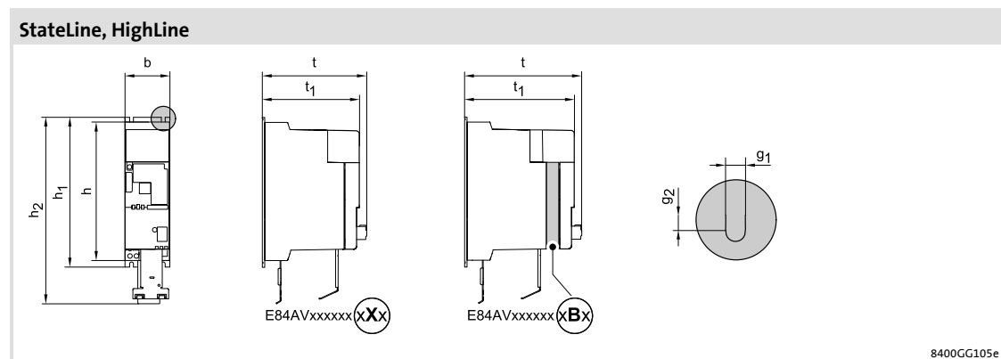
Fig. 5-15 Device dimensions
