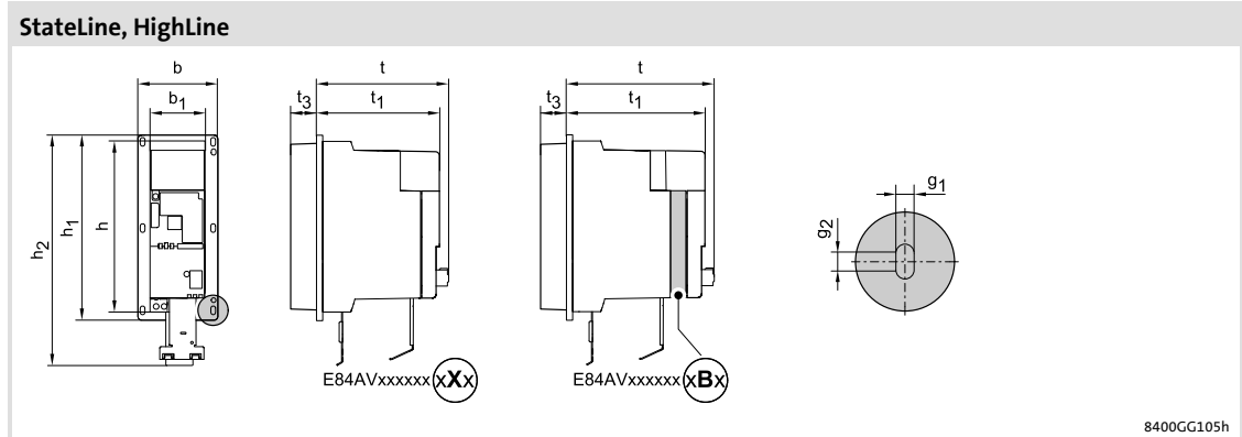
Fig. 5-7 Device dimensions
