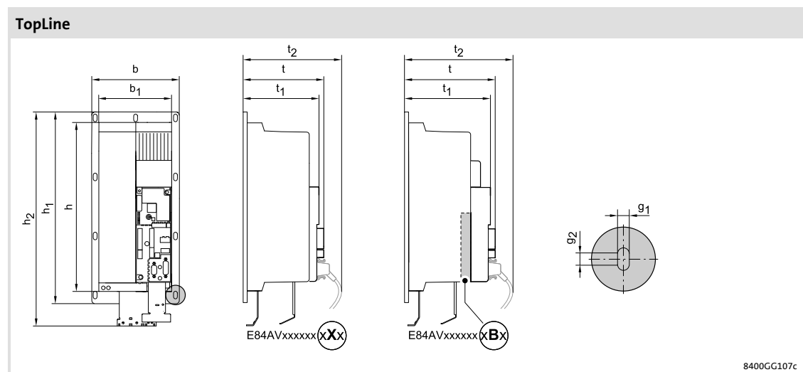
Fig. 5-39 Device dimensions
