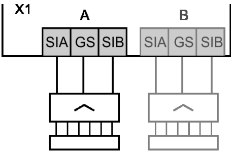
Connection of Basic Safety STO safety system
