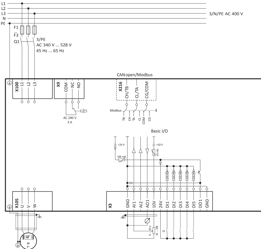
Fig. 11: Wiring example
