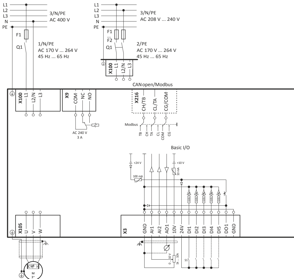
Fig. 8: Wiring example
